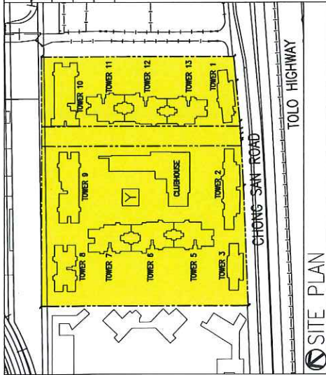
LOCATION PLAN OF AIR-CONDITIONER OUTDOOR UNIT(S)
