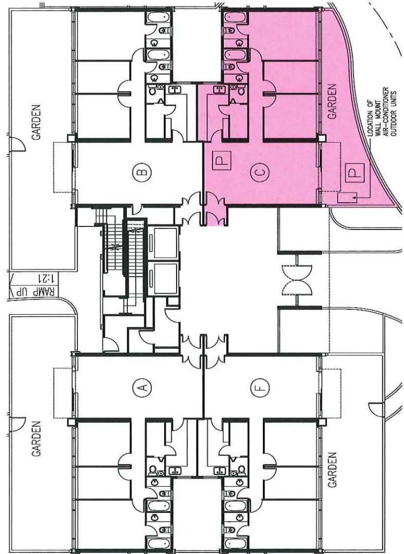
TOWER 8 GROUND FLOOR PLAN
